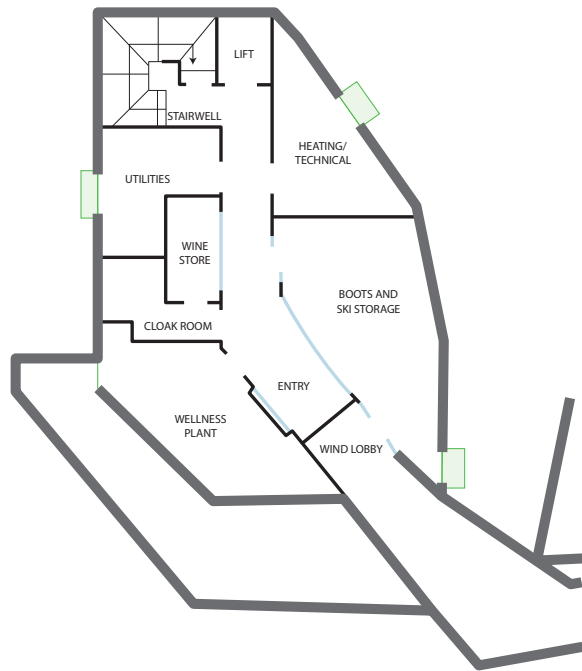
BASEMENT LEVEL AND ENTRANCE PLAN
